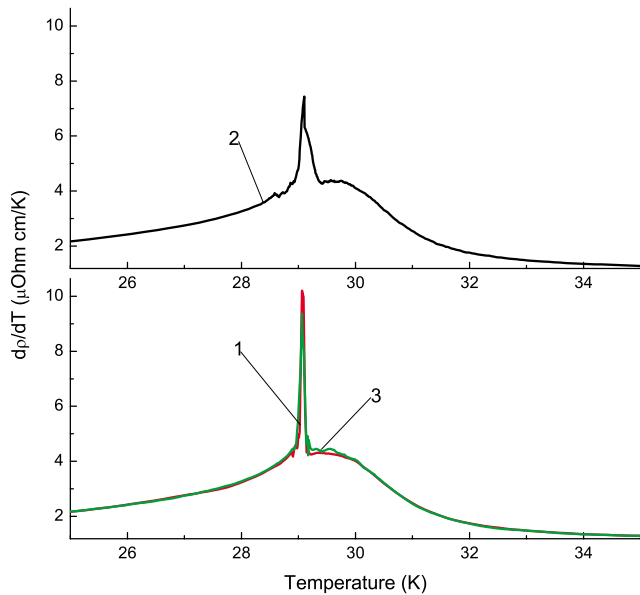
FIG. 6. (Color online) Influence of fast pressure releasing on the peak of dp/dT at the phase transition in MnSi. 1—ambient pressure, 2—ambient pressure after loading the sample to 1.2 GPa, and 3—after holding the sample experienced 1.2 GPa for a week at ambient pressure.
