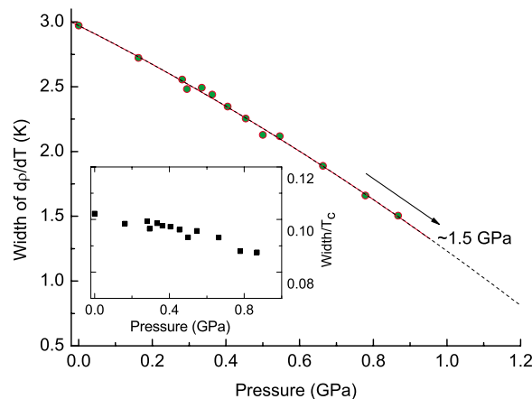
FIG. 5. (Color online) Pressure dependence of the width of the global maximum in d\rho/dT . The inset shows small variation in the ratio width/temperature with pressure. The width is taken at the level of 3 \mu\text{Ohm cm/K} (see Fig. 3). Note that the melting curve of helium and the phase-transition line are crossed at about 0.27 GPa.
