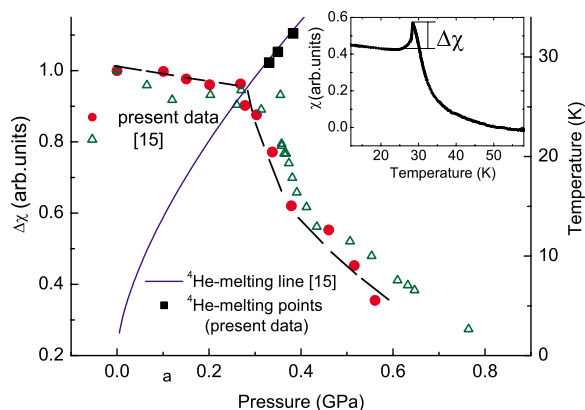
FIG. 2. (Color online) Evolution of the form of \chi_{ac} at the phase transition in MnSi. The definition of \Delta\chi is given in the inset.
